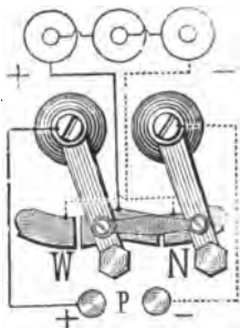
Current reverser.
